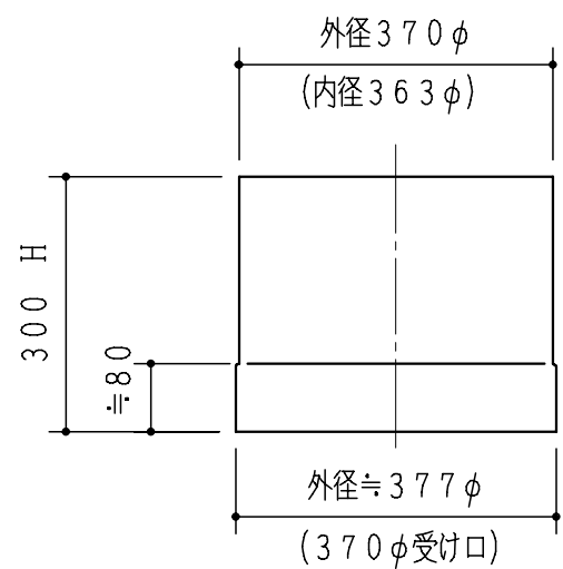
370φ×300H (PVC製)
