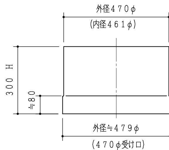
450φ×300H (PVC製)
